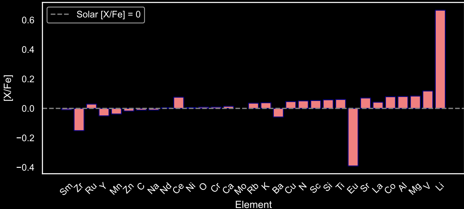
Abundance Pattern for GALAH Main Sequence Stars: Star Field [66] (N=130)
