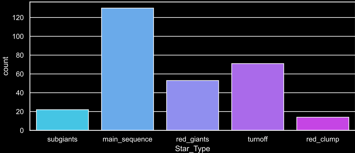
Field [66] Count plot of Star Type
