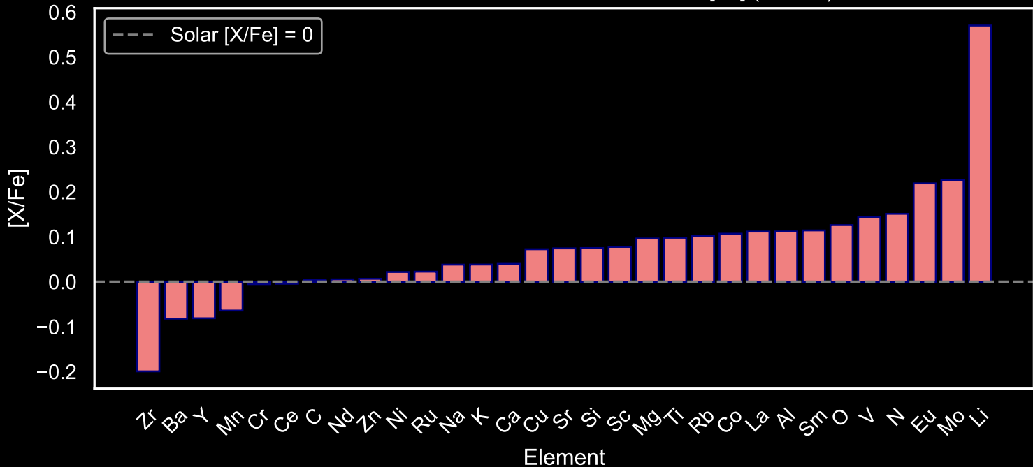
Abundance Pattern for GALAH Star Field [66] (N=290)
