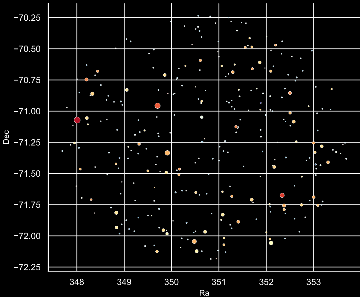
Field [66] Ra [350.8] Dec [-71.23] Stars: 290
