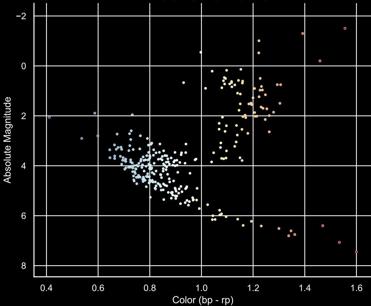
GALAH Hertzprung-Russel Diagram Field [66] Ra [350.8] Dec [-71.23]
