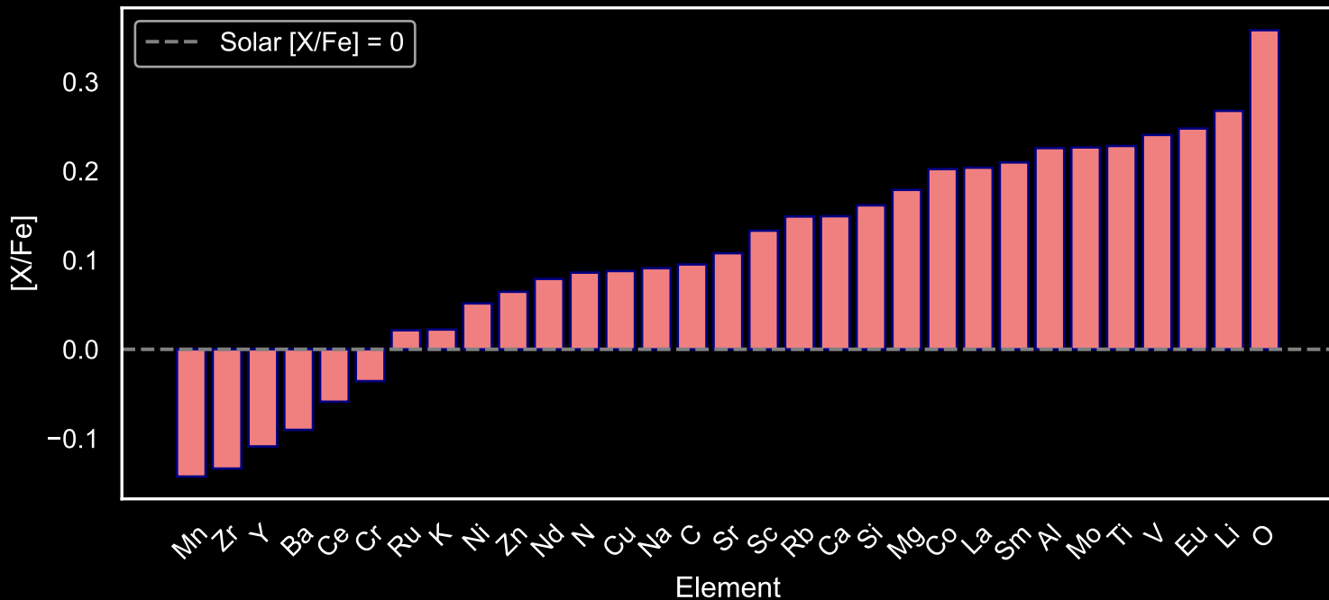
Abundance Pattern for GALAH Red Giants: Star Field [66] (N=67)
